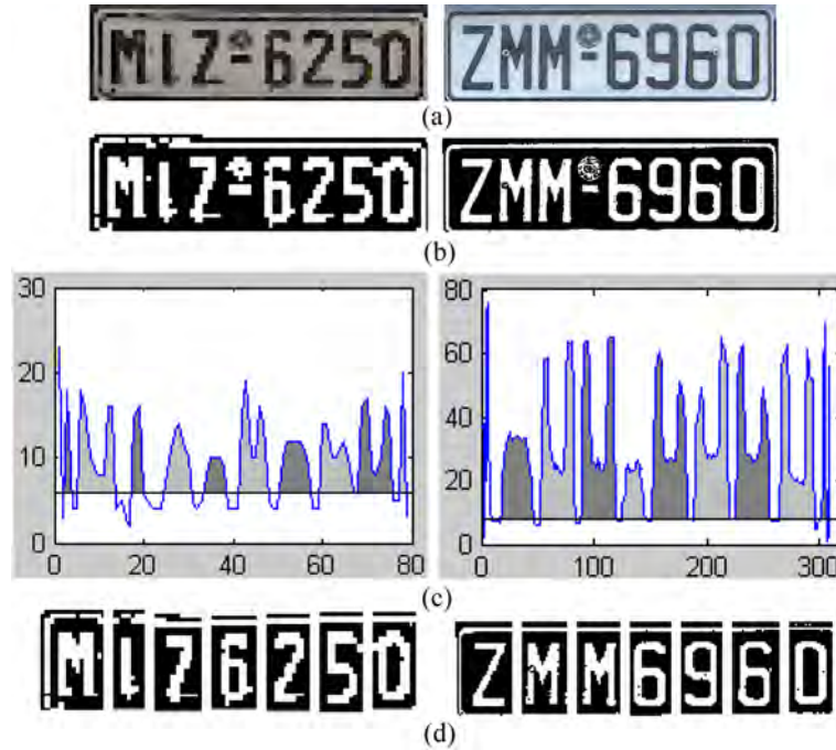
Fig. 5.4: License plate segmentation: (a) Original license plate, (b) Inverted binary images, (c) Vertical projections, and (d) Segmented characters and digits.
