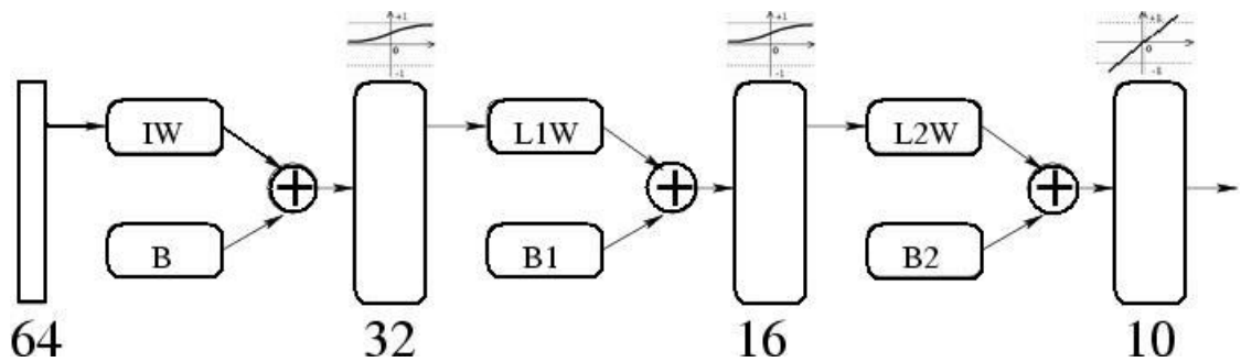
Fig. 4.10: Neural network for digit classification.
