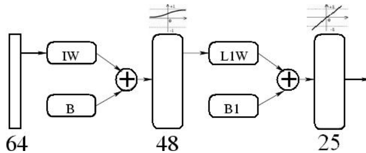
Fig. 4.11: Neural network for character classification.
