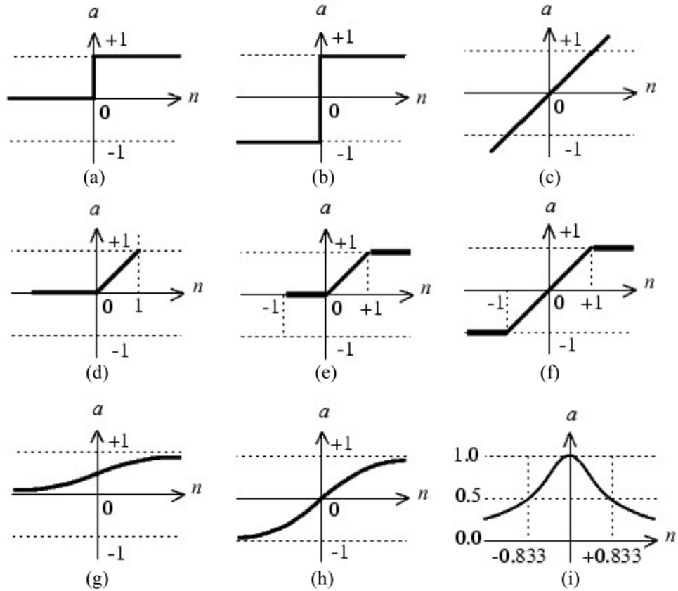
Fig. 2.9: Activation functions: (a) Hard limit, (b) Symmetric hard limit, (c) Pure linear, (d) Positive linear, (e) Saturating linear, (f) Symmetric saturating linear, (g) Log sigmoid, (h) Tan sigmoid, and (i) Radial basis.
