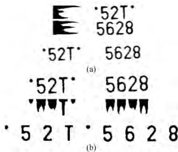
Fig. 3.5: The license plate segmentation stage [4]: (a) Row segmentation using horizontal projection, and (b) Character segmentation using vertical projection.
