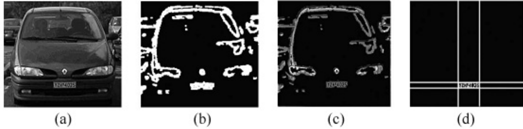
Fig. 3.1: Steps for license plate segmentation: (a) Original image, (b) Result of SCW segmentation technique after the application of the segmentation rule and thresholding, (c) Image after logical AND operation, and (d) License plate detection.
