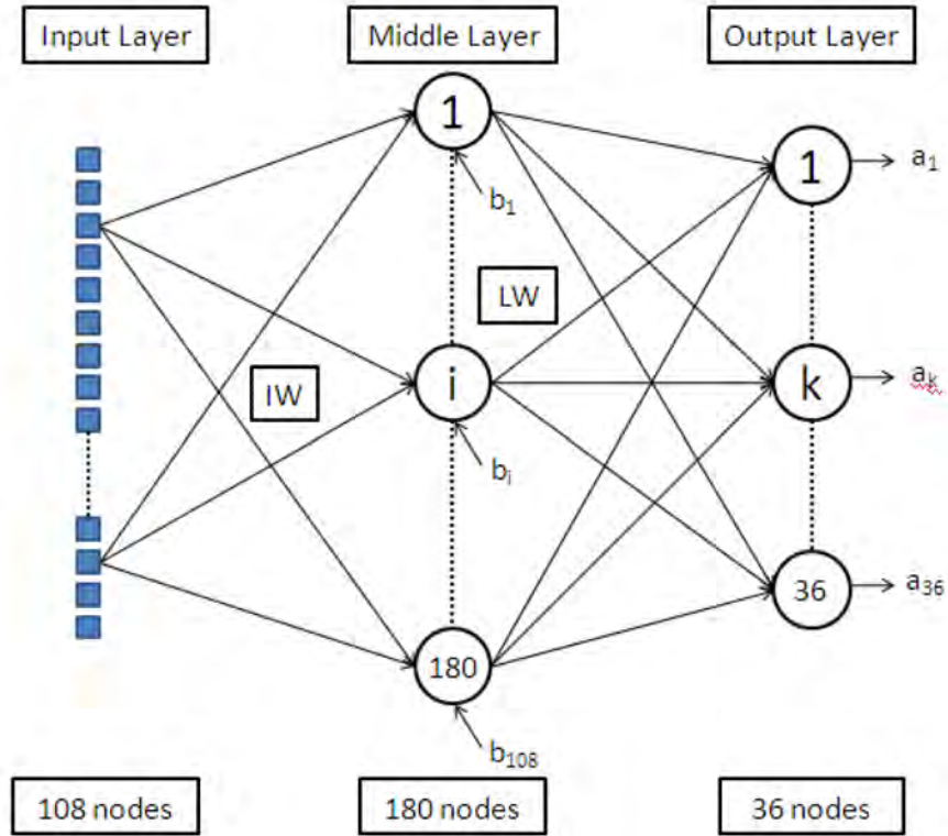
Fig. 3.3: Architecture of the PNN [3].
