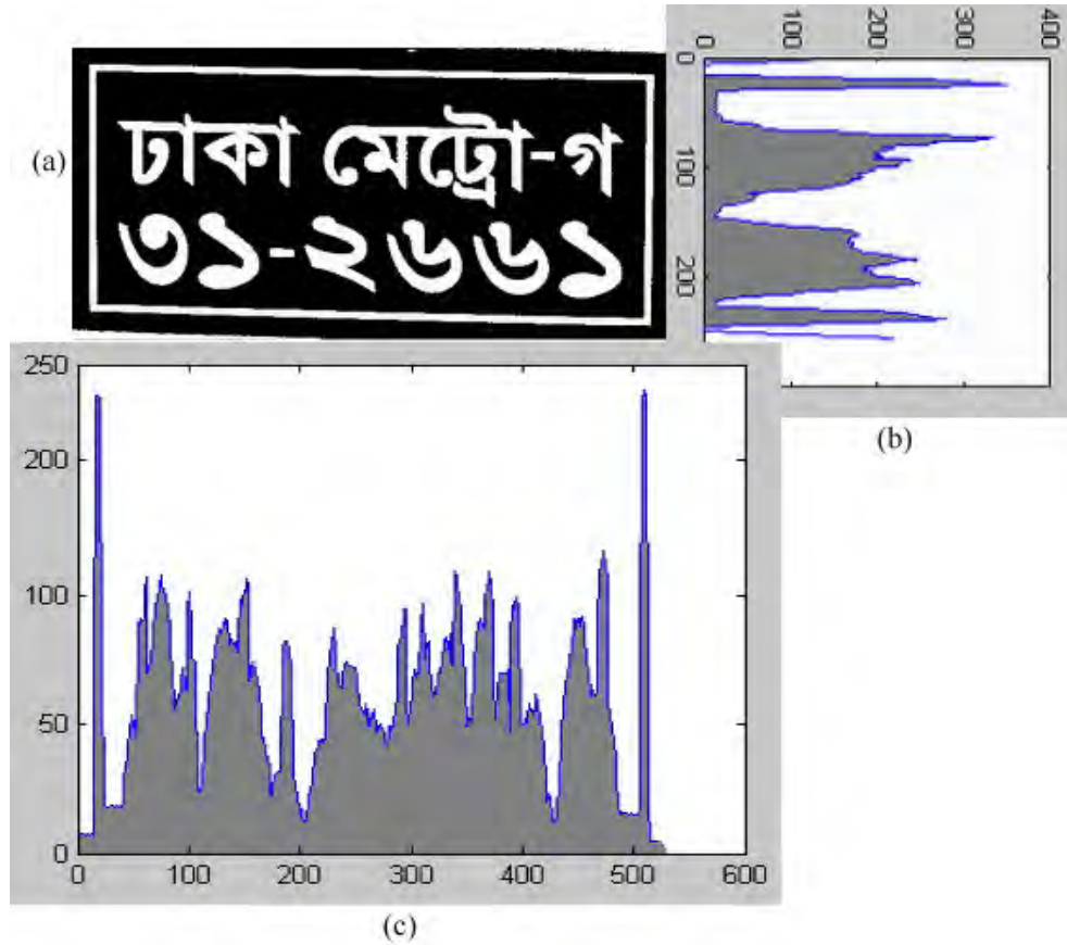
Fig. 2.6: (a) Original license plate image, (b) Horizontal projection, and (c) Vertical projection.
