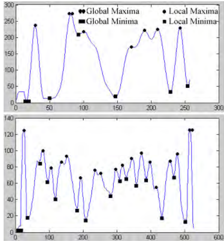
Fig. 2.8: Extrema detection.
