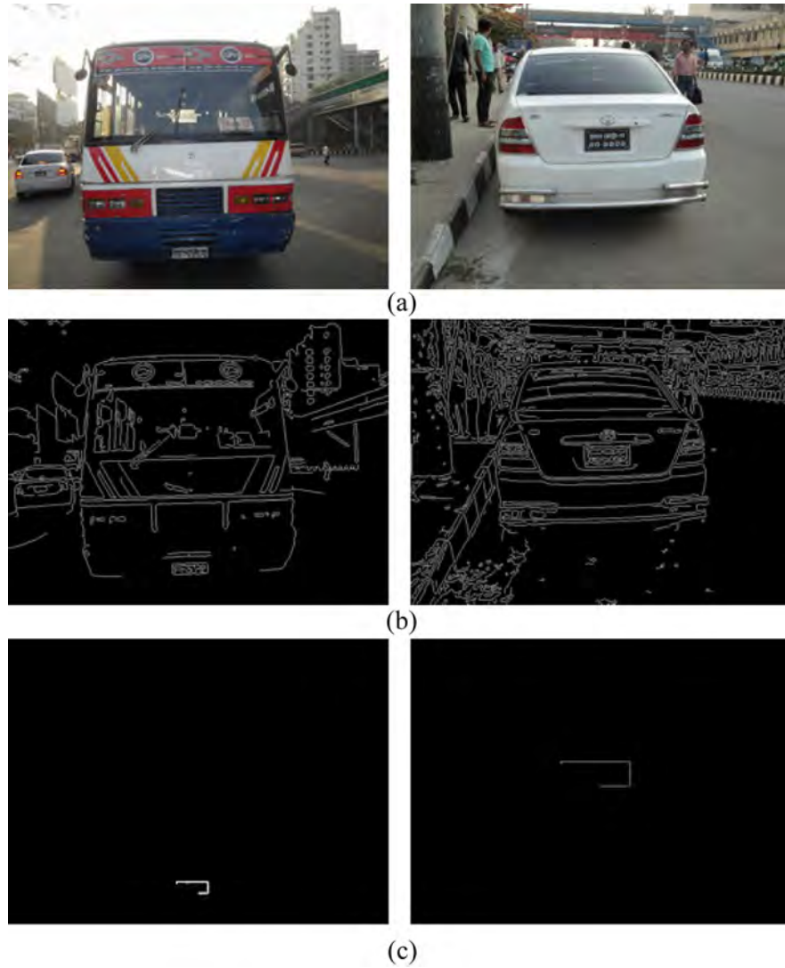
Fig. 5.1: License plate detection: (a) Original input images, (b) Edge images, and (c) After the application of symmetry detection algorithm and ROI.
