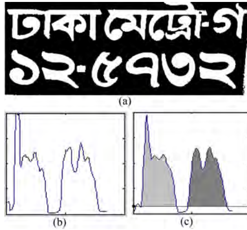
Fig. 4.2: Sample outputs of license plate segmentation stage: (a) Binary image of a simple license plate, (b) Horizontal projection of the pixels, and (c) Filtered projection.
