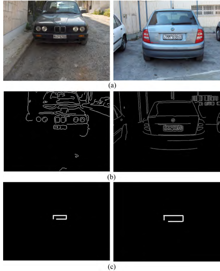
Fig. 5.3: License plate detection: (a) Original input images, (b) Edge images, and (c) After the application of Algorithm ROID.
