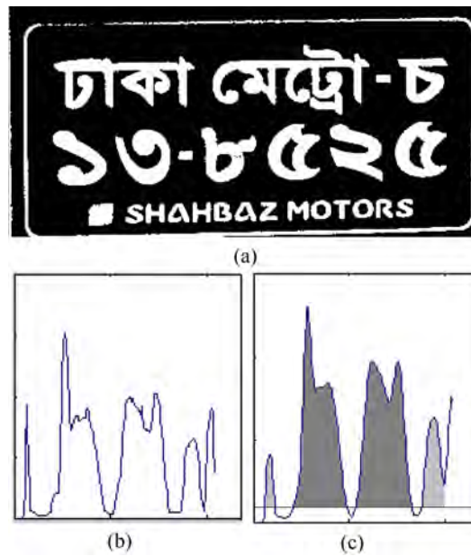
Fig. 4.3: Sample outputs of license plate segmentation stage: (a) Binary image of a complex license plate, (b) Horizontal projection of the pixels, and (c) Filtered projection.
