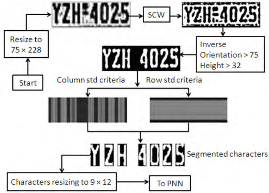
Fig. 3.2: Flowchart indicating the license plate segmentation process [3].
