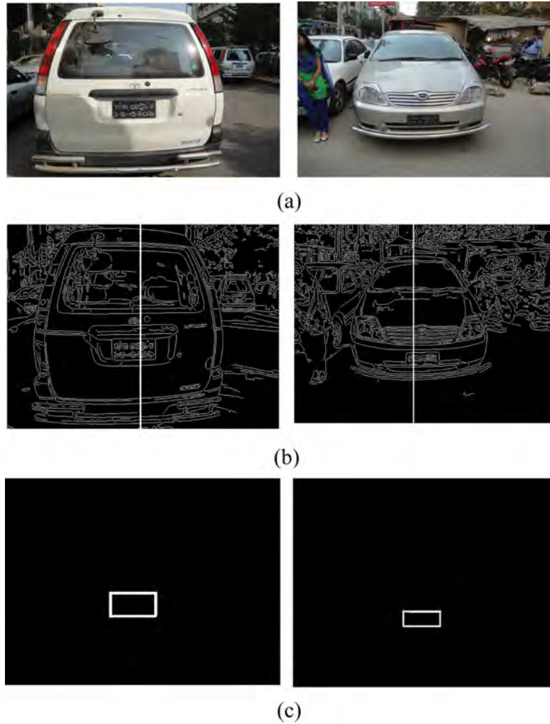
Fig. 4.1: Sample outputs of license plate detection stage: (a) Input image containing vehicle, (b) Edge image with overlaying vertical axis of symmetry, and (c) Detected ROI.
