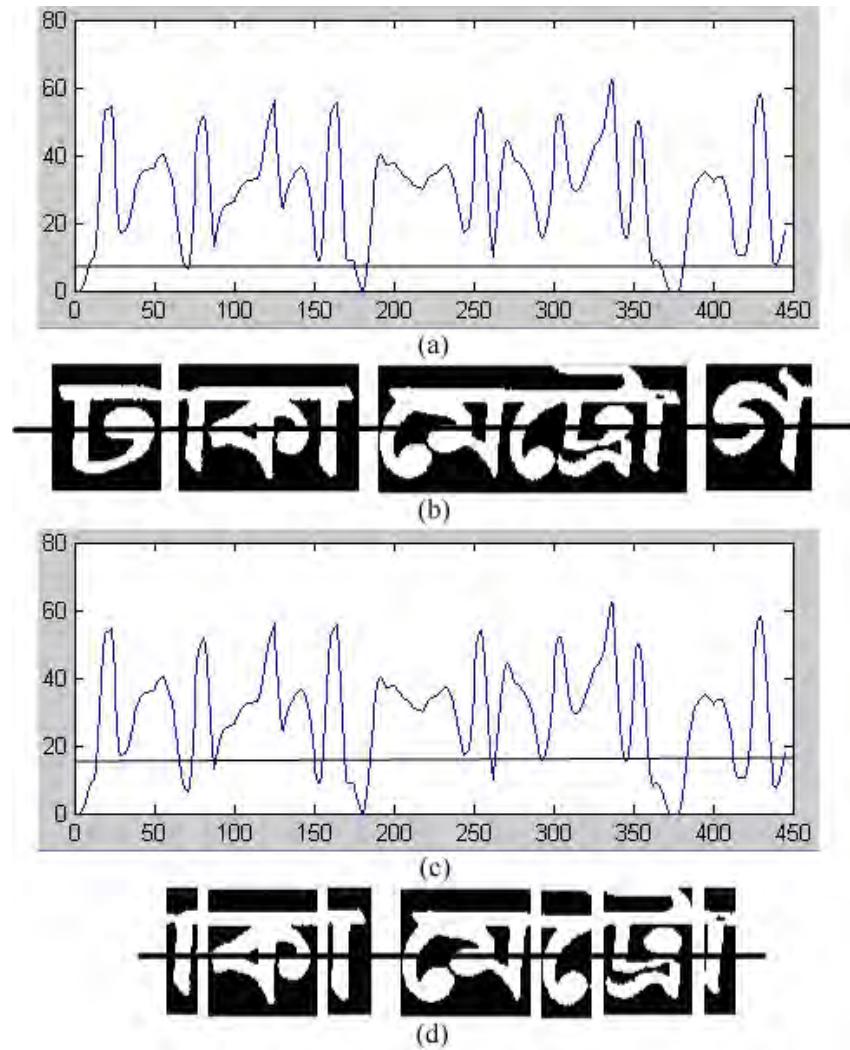
Fig. 4.6: Segmenting characters
