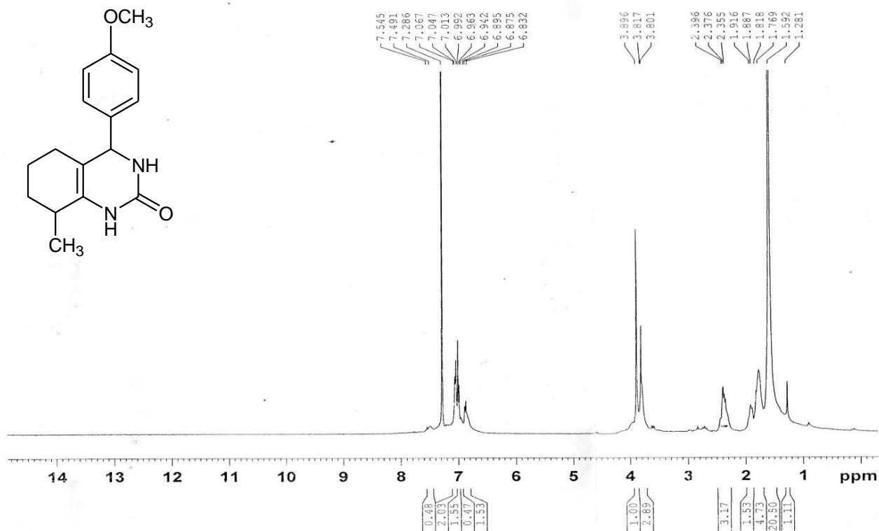
Fig 14 : 1 H-NMR Spectrum for Compound (1)
